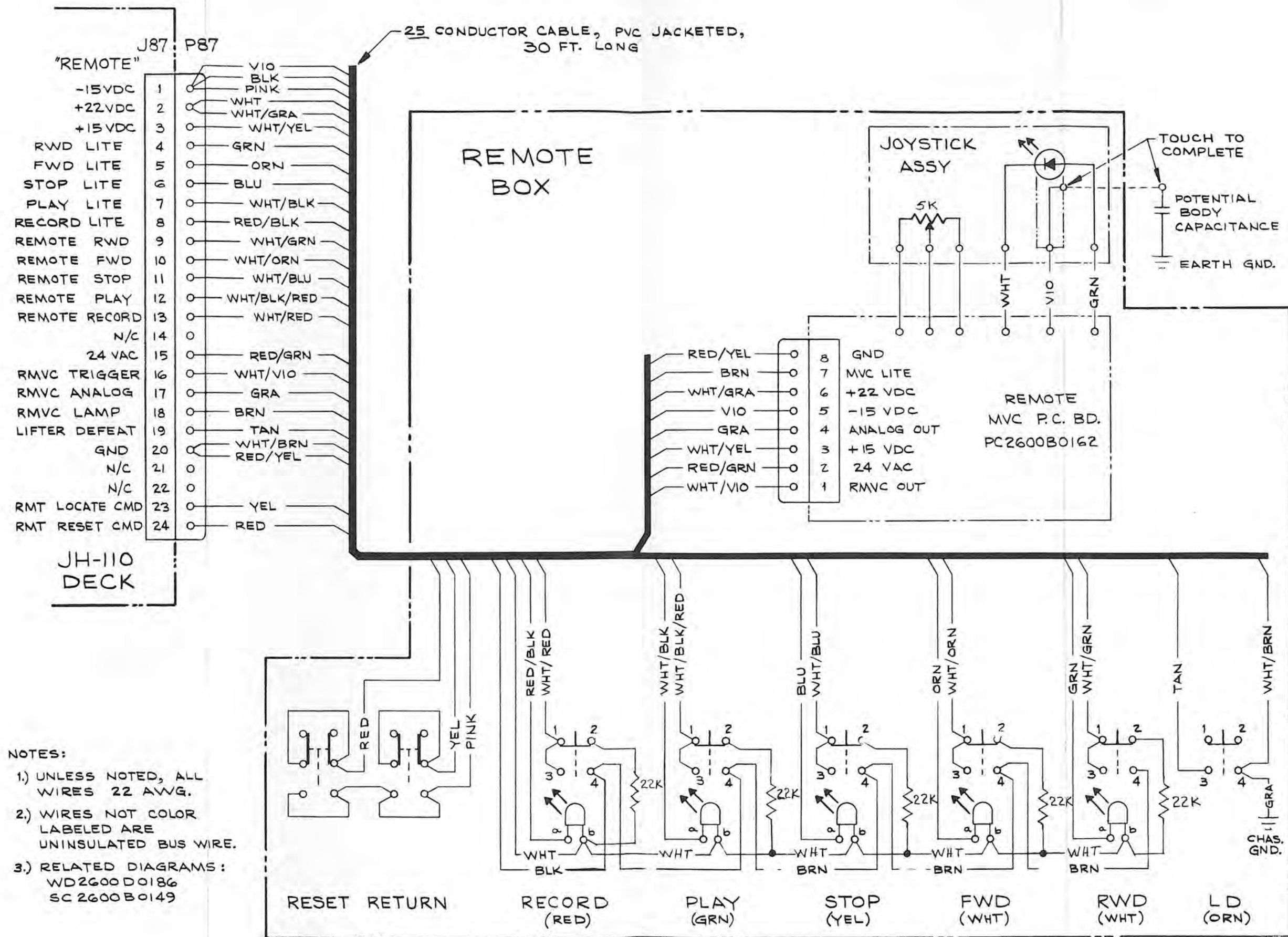
Remote Box & Cable 26C150 JH-110A
