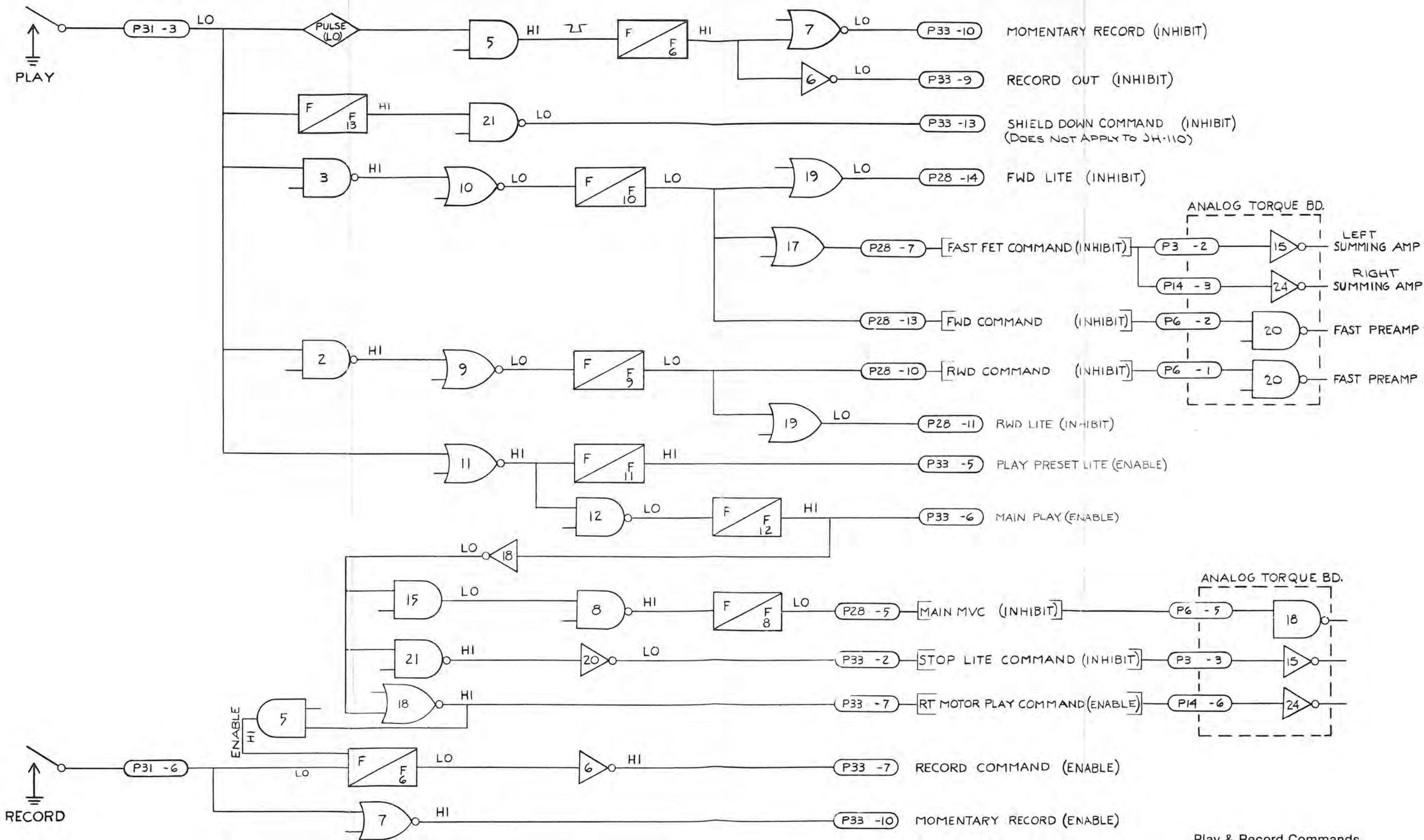
Figure 15 Play & Record Commands JH-110A Page 3-13
