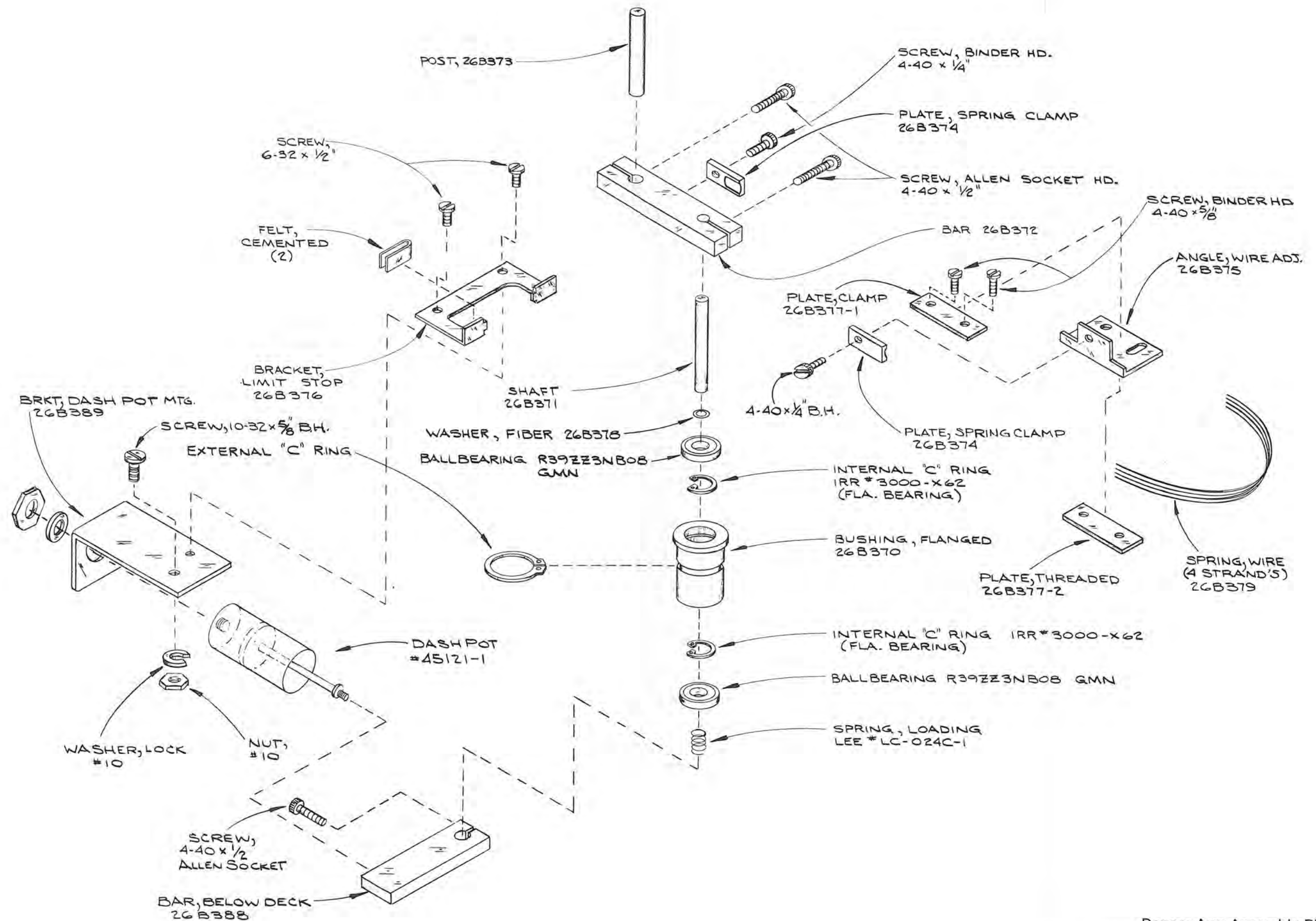
Figure 84 Dancer Arm Assembly Pictorial JH-110A Page 10-47
